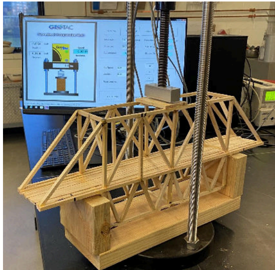
Figure 1: Loading Configuration
